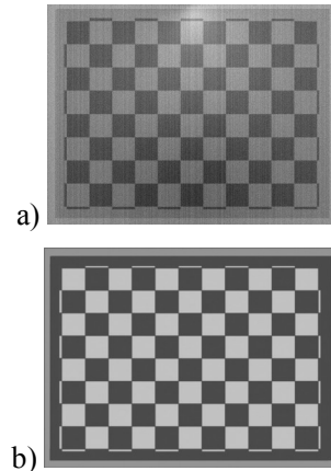
Fig. 2. Image of FUT target generated by: a) thermal imager, b) visible camera
